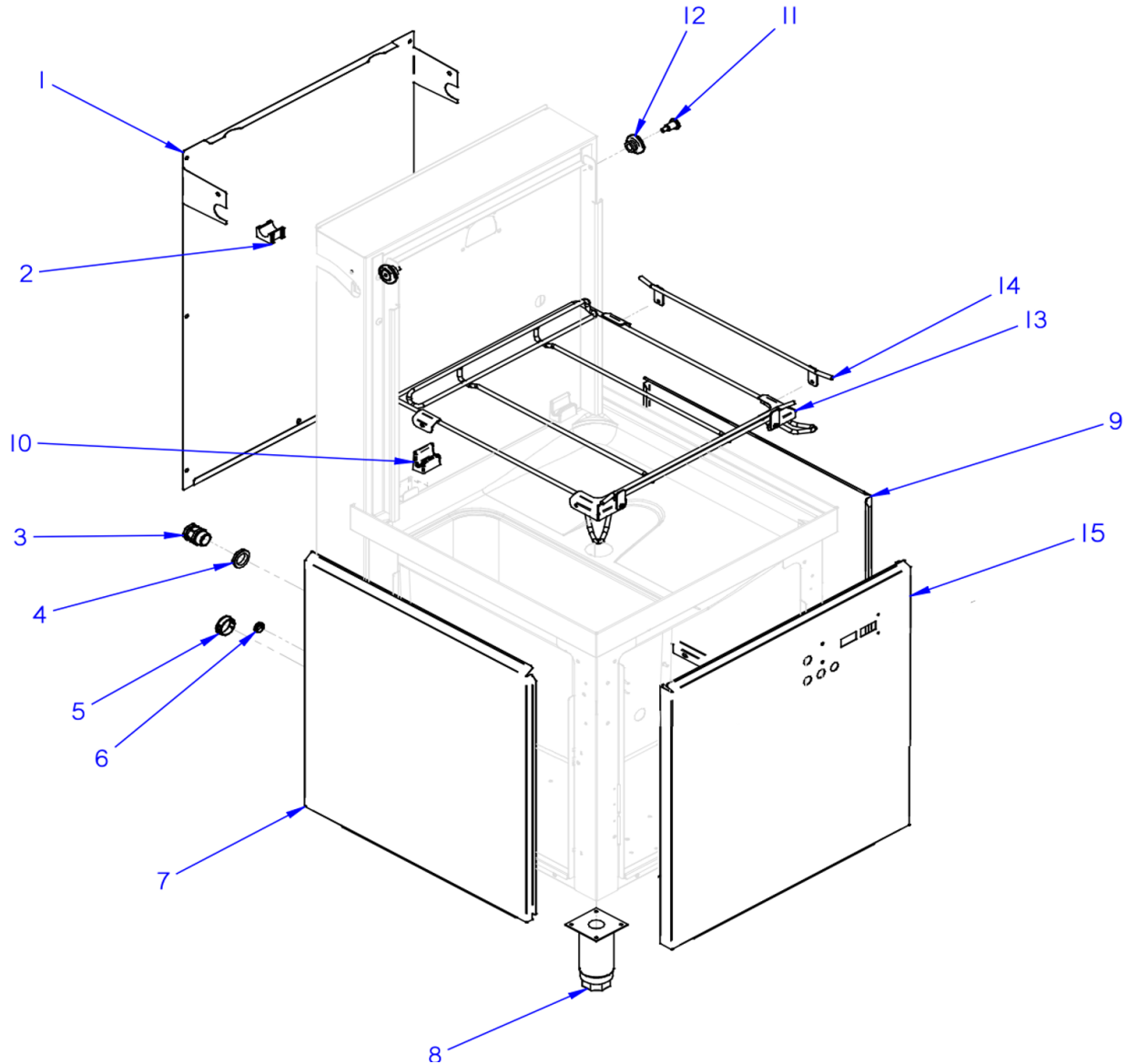
FIGURE 1 CABINET OF THE MACHINE
