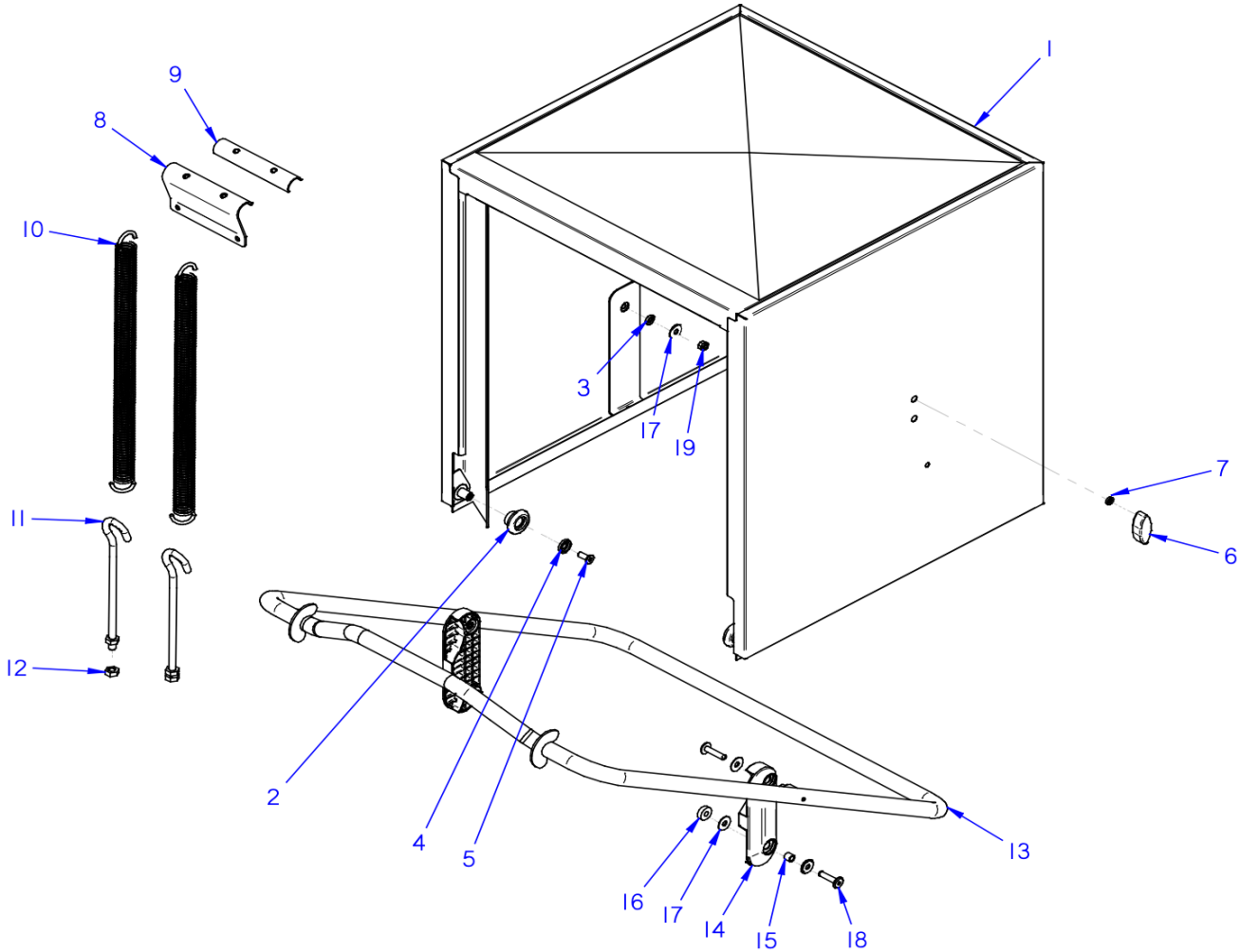
FIGURE 2 HOOD
