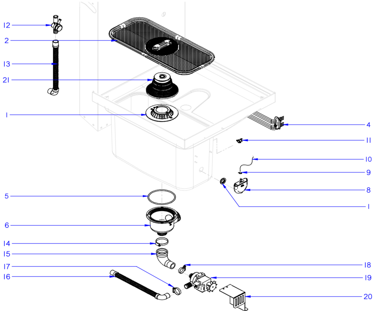
FIGURE 3 TANK PARTS
