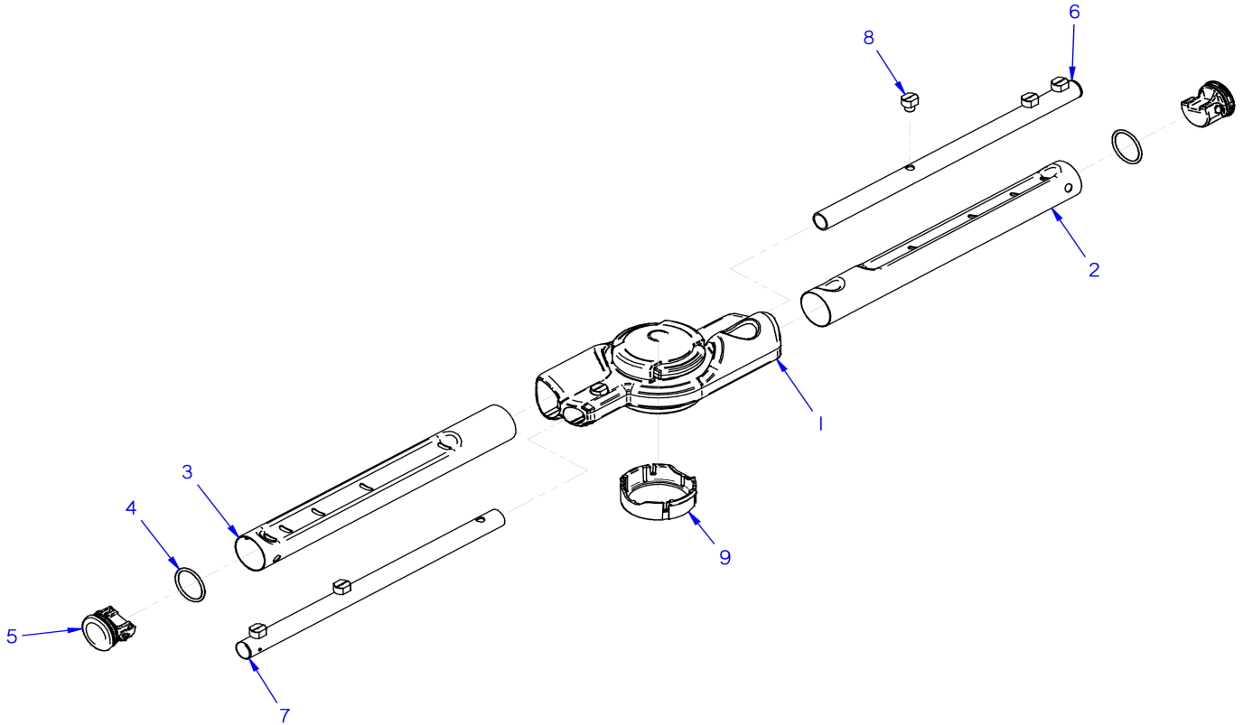
FIGURE 7 SS DISPENSER(OPTIONAL)
