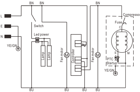
CIRCUIT DIAGRAM
