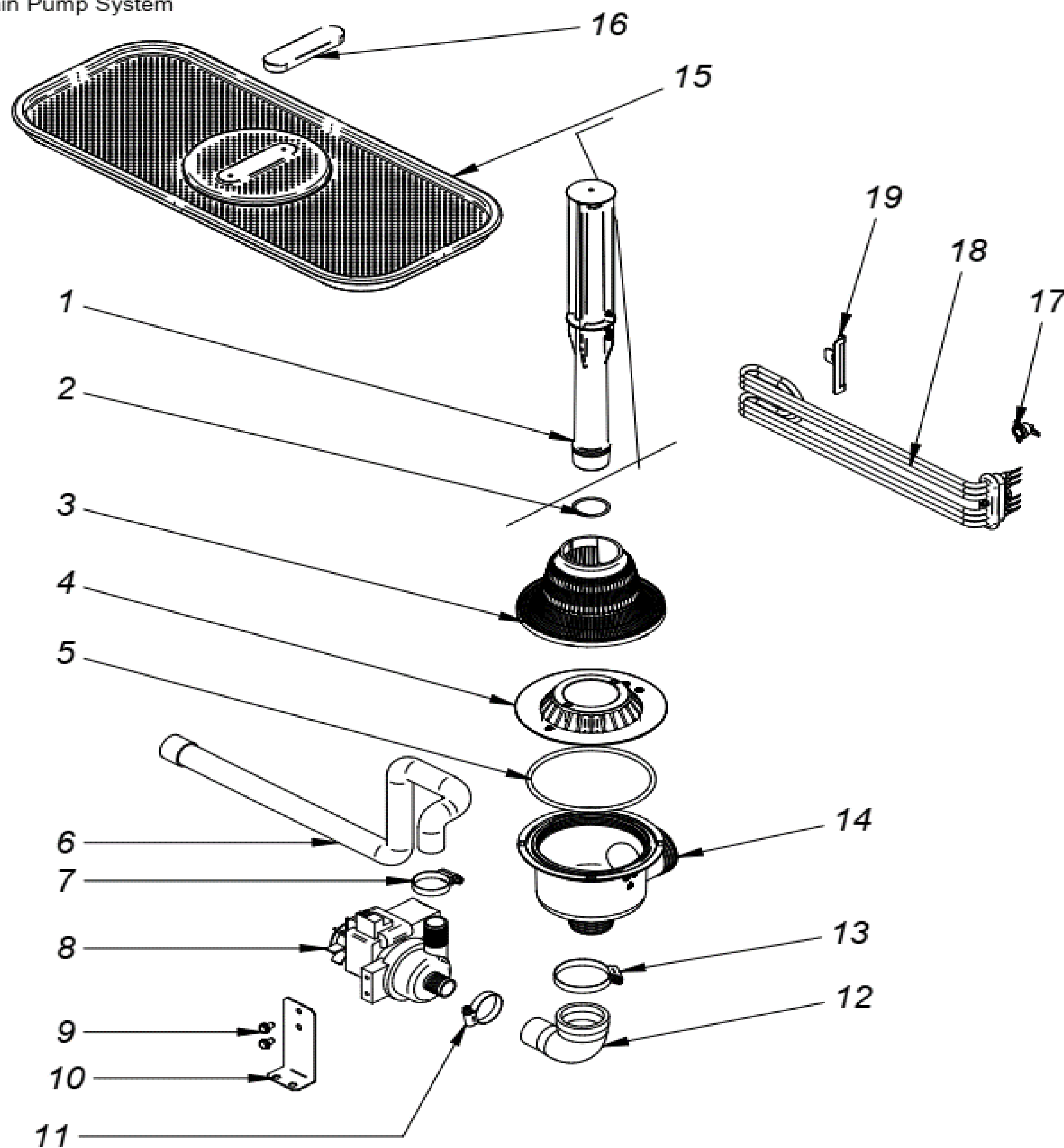
Drain Pump System
