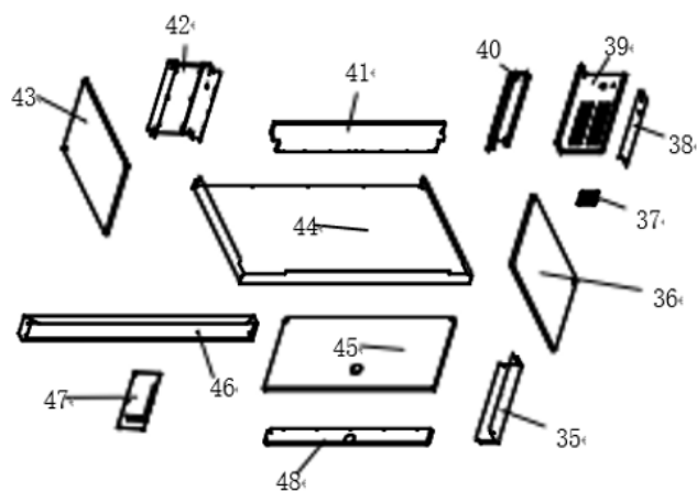
Outer Case
