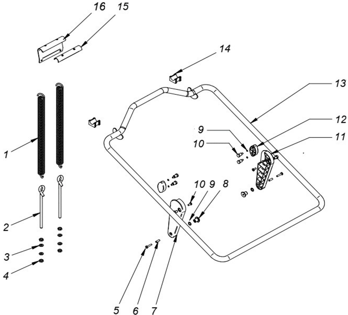
FIGURE 2 TILTING SYSTEM
