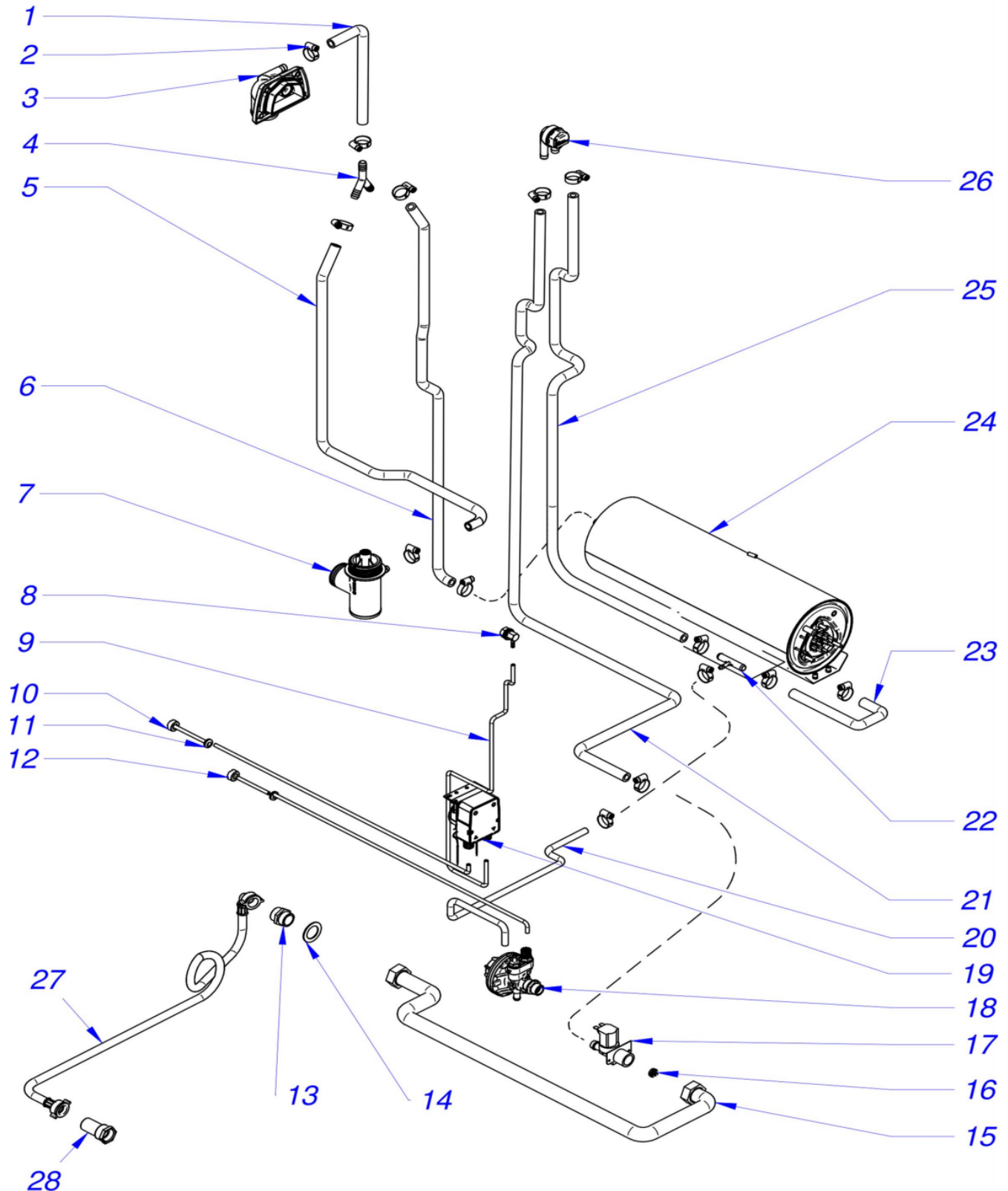
FIGURE 4 HYDRULIC SYSTEM
