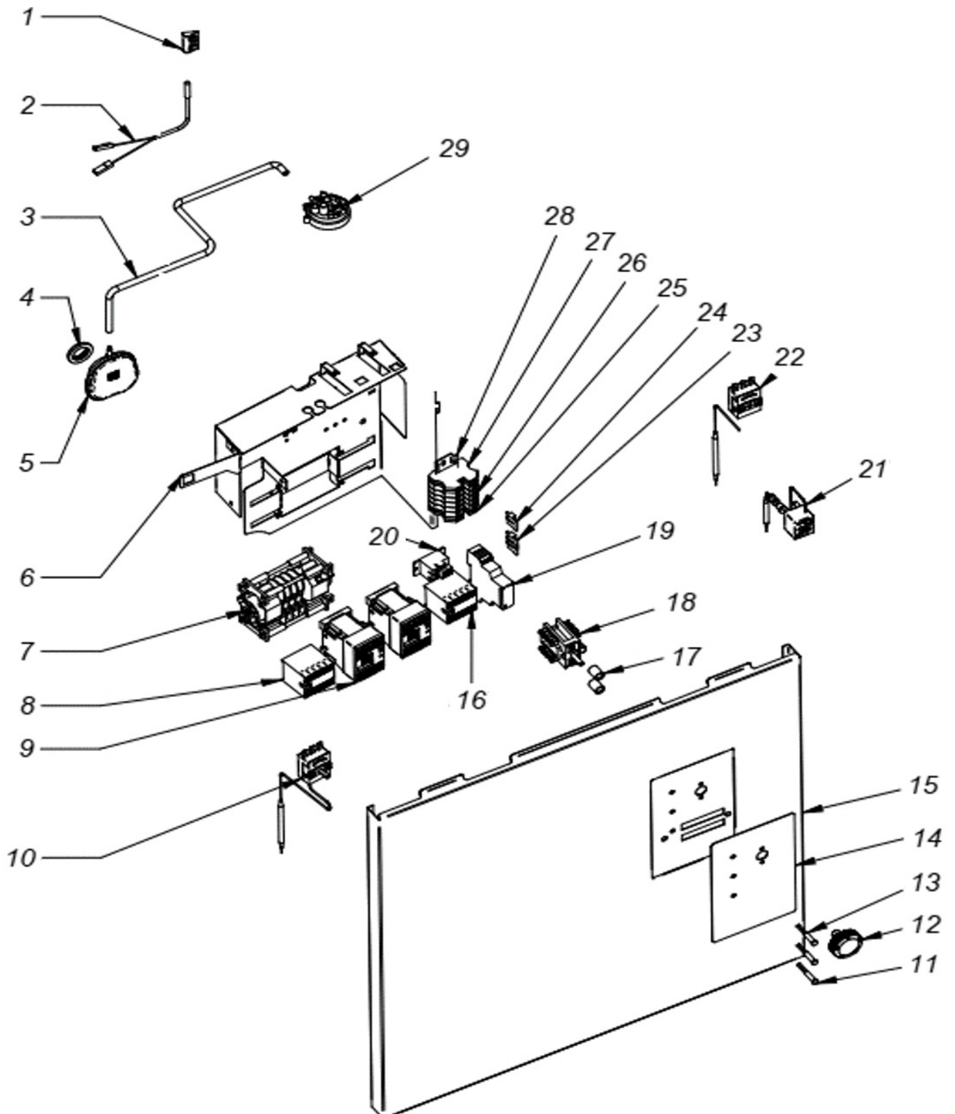
FIGURE 8 ELECTRIC SYSTEM
