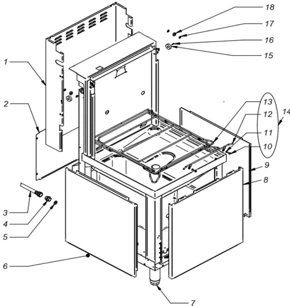
FIGURE 1 MAIN BIEW OF THE MACHINE
