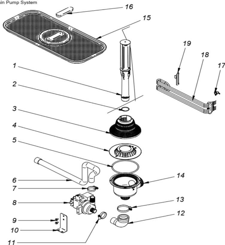
Drain Pump System
